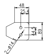
LV BUSHING TERMINAL DETAIL
