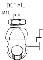
HV BUSHING TERMINAL DETAIL
