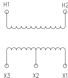
LV BUSHING TERMINAL DETAIL
